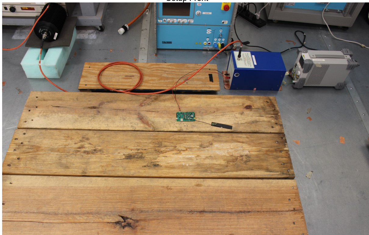
Setup Front
